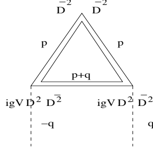
Figure 7: Relevant diagram for the Konishi anomaly
