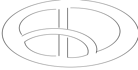
Figure 6: A non-planar genus g = 1 diagram
