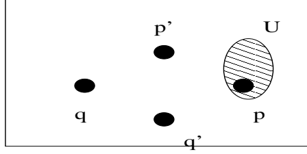
Figure 3: A sketch of a two-dimensional mass hyperboloid with four scattering states satisfying p + q = p' + q' . If p is outside the region U then this state is annihilated by f \cdot A .
