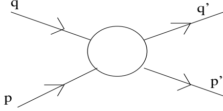
Figure 2: Scattering of two particles with momentum p and q into two particles with momentum p' and q' .
