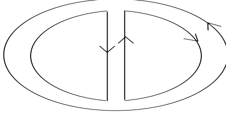
Figure 5: A planar diagram with vertices of degree 3. The double line notation indicates that the fields are in the adjoint representation with each line representing one index of \phi_{ij}
