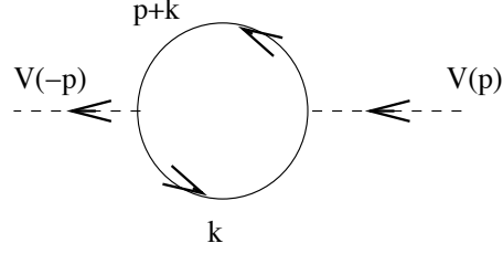
Figure 4: Feynman diagram for vacuum polarisation
