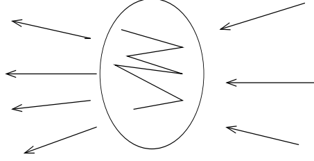
Figure 1: n-particle scattering
