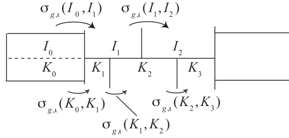
Figure 5. The boundary condition for t -leaf segments.
