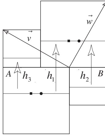
Figure 7. The complete set of holonomies \mathcal{H} = \{h_1, h_2, h_3, h_1^{-1}, h_2^{-1}, h_3^{-1}\} for the Anosov map g : \mathbf{R}^2 \setminus (\mathbf{Z}\bar{v} \times \mathbf{Z}\bar{w}) \rightarrow \mathbf{R}^2 \setminus (\mathbf{Z}\bar{v} \times \mathbf{Z}\bar{w}) defined by g(x, y) = (x + y, y) and with Markov partition \mathcal{P} = \{A, B\} .
