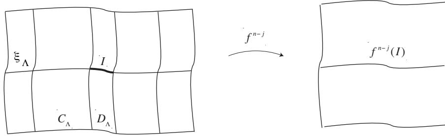
Figure 11. The (n - j + 1) -cylinder leaf segment I = \xi_\Lambda \cap D_\Lambda and the primary leaf segment f^{n-j}(I) = i(\pi_{\iota'} \tau_i^{n-j}(\xi \cdot D)) , where D = m_i^{j-1} C .
