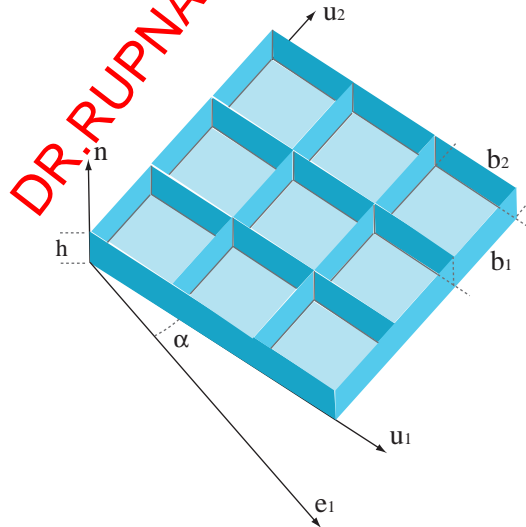
Figure 9. Geometry of microcubicles.
